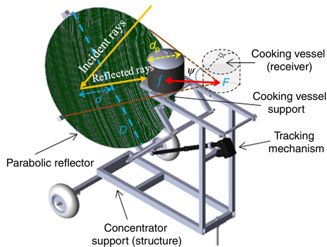
Fig. 5 A 3D View of the new configuration design for parabolic solar cooker
