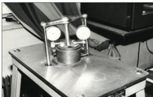
Figure 3. Swelling test in an oedometer under load.
