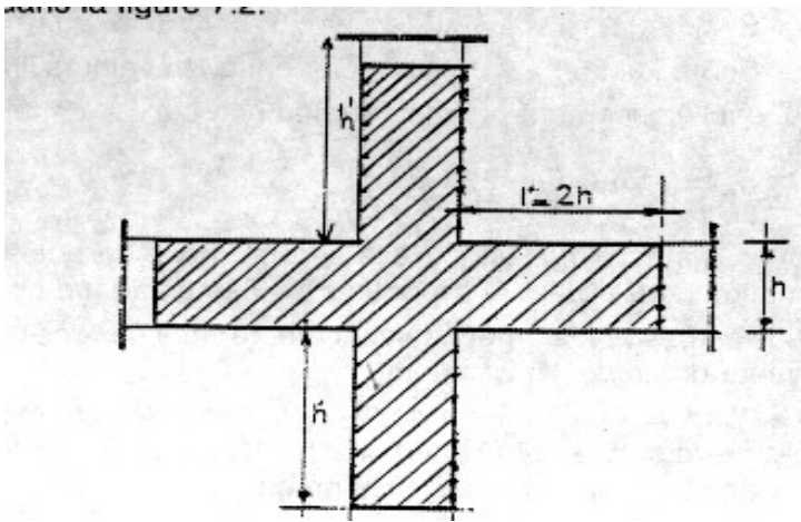
h' = \text{Max}(h_e/6; b_1; h_1; 60) FIG. 7.2 : zone nodale
